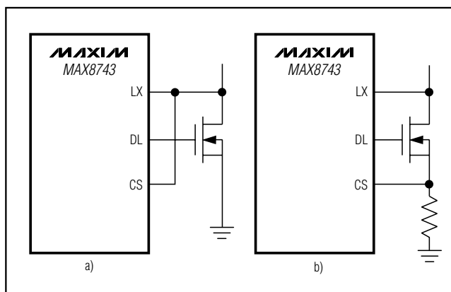
Figure 7. Current-Sense Configurations
